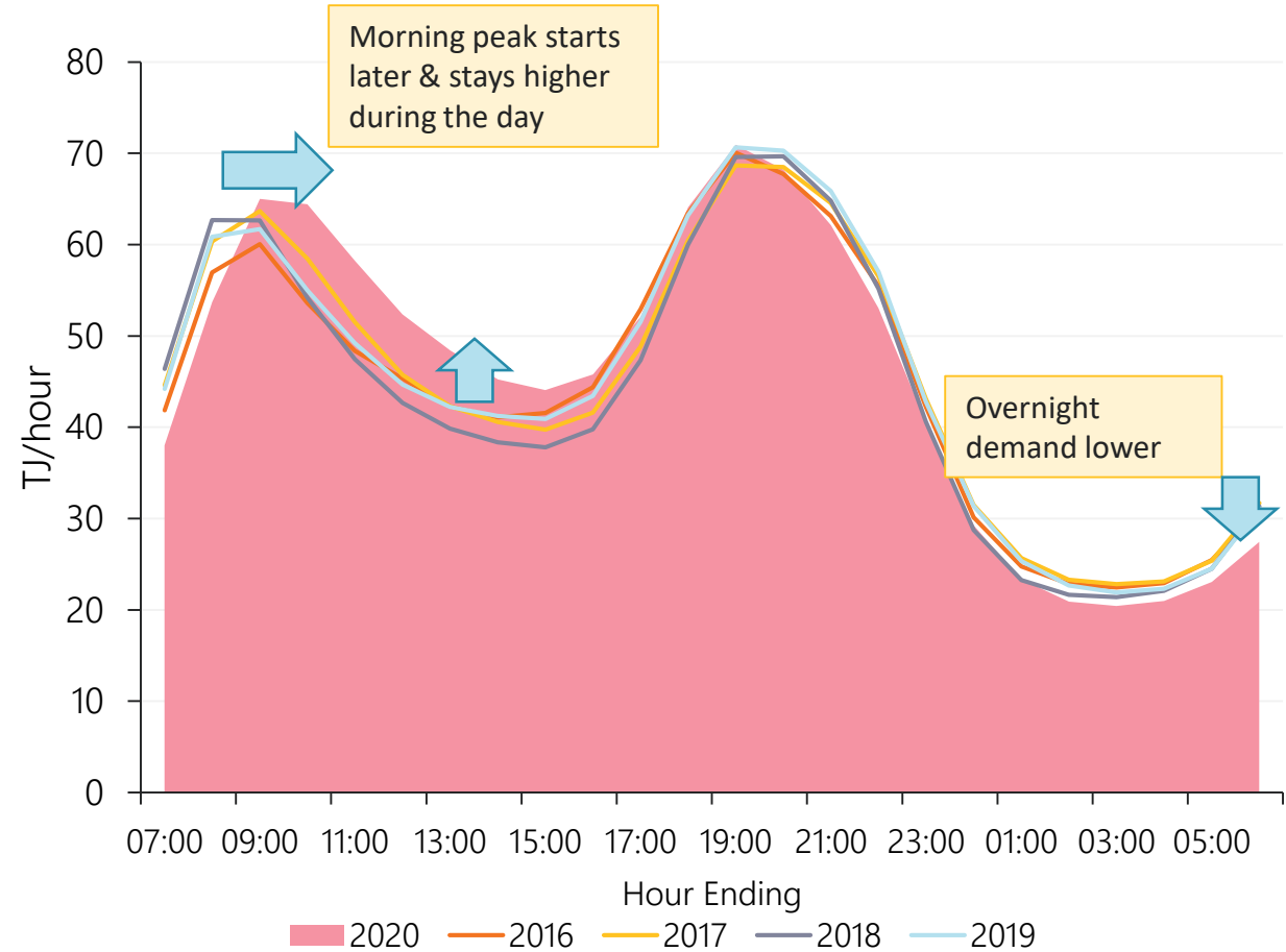
Higher demand during day on cold days
