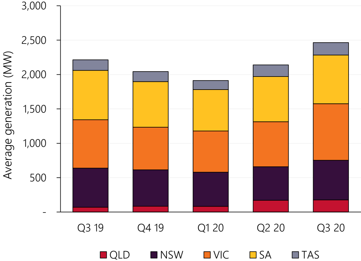
Quarterly wind output reached record levels
