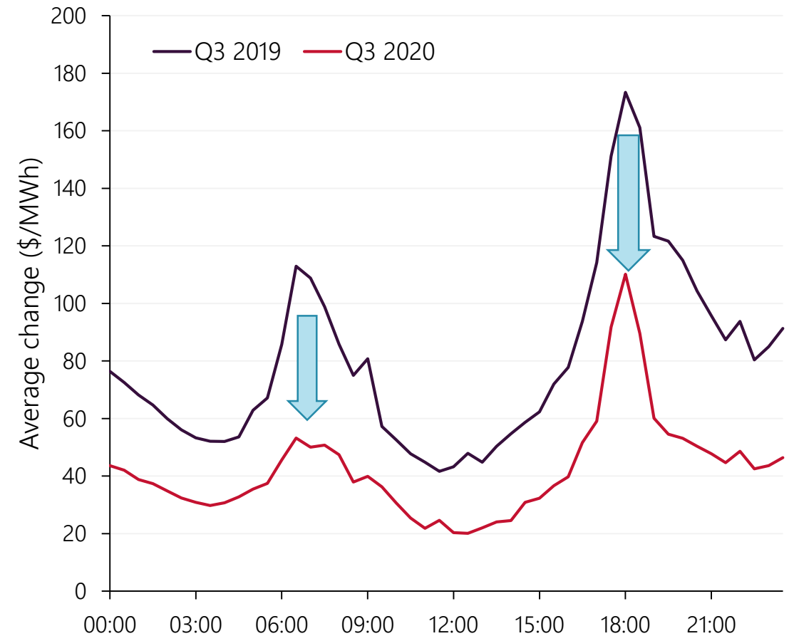
Largest spot price reductions during the evening peak
