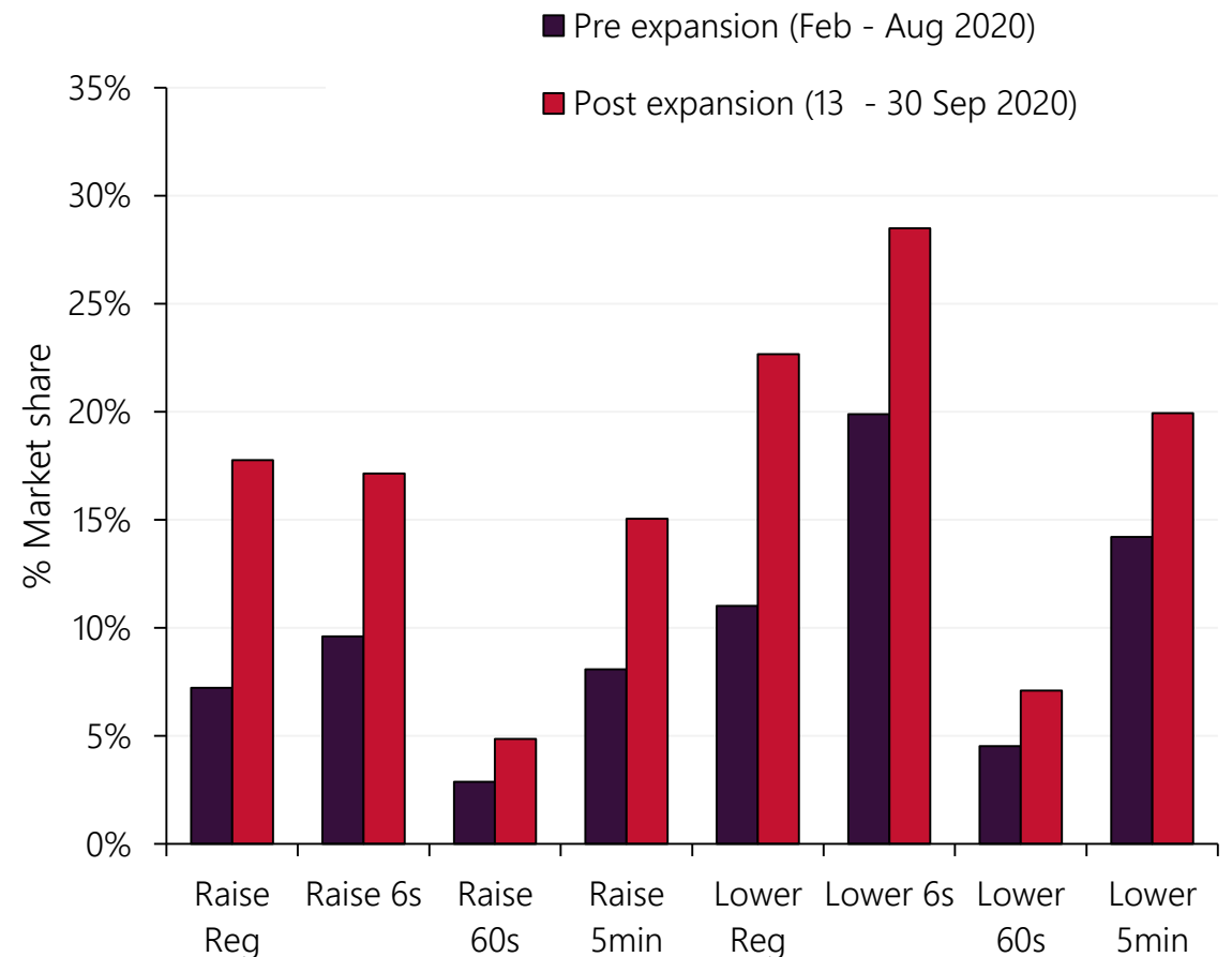
Hornsdale battery captures 17% of NEM wide FCAS market share following expansion
