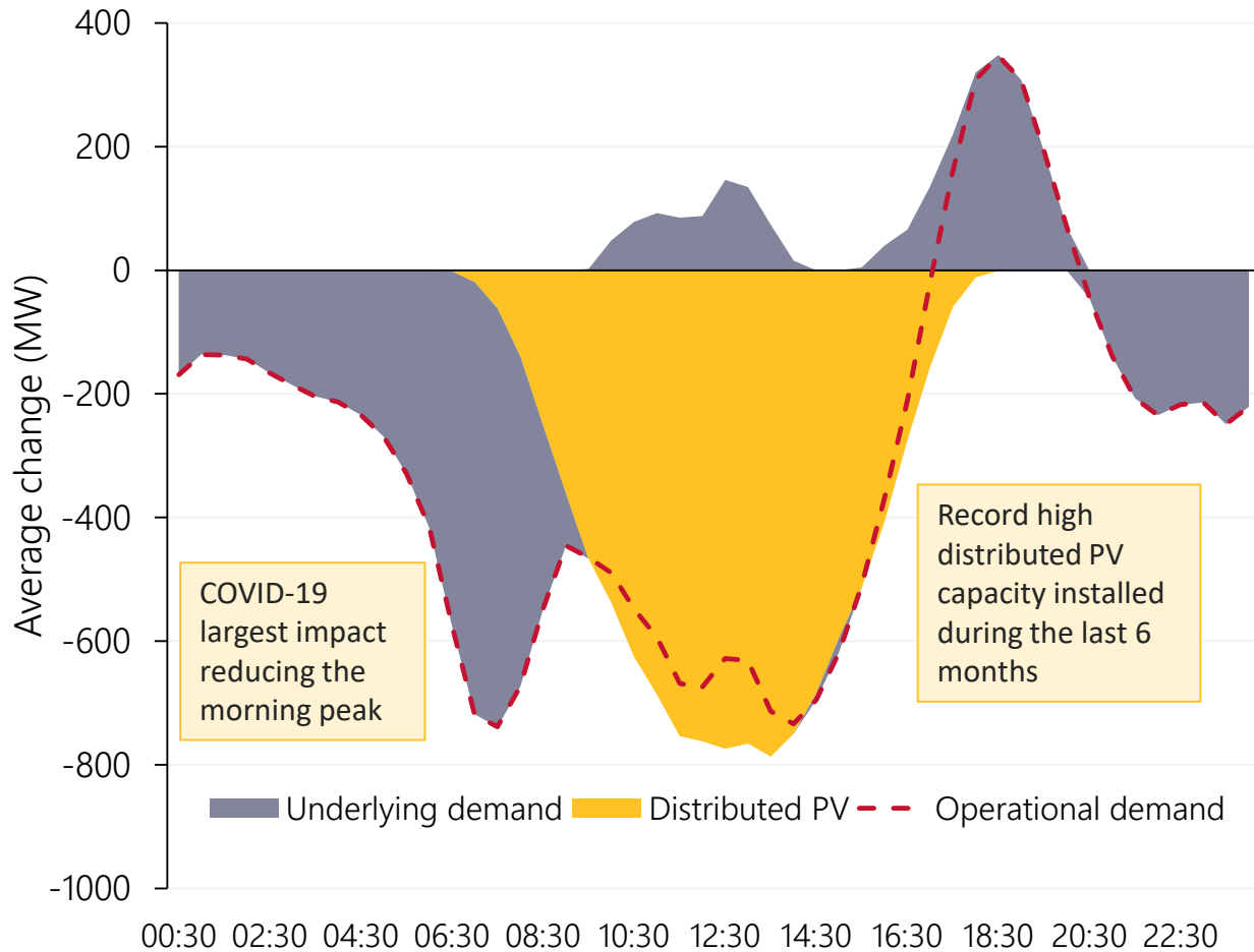
NEM operational demand down 1.4%
