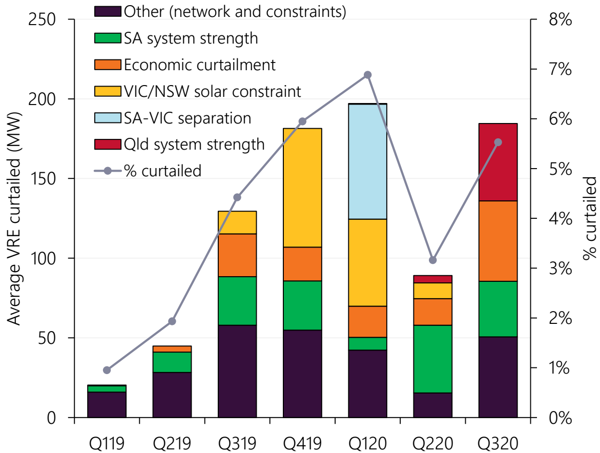
VRE curtailment on the rise again
